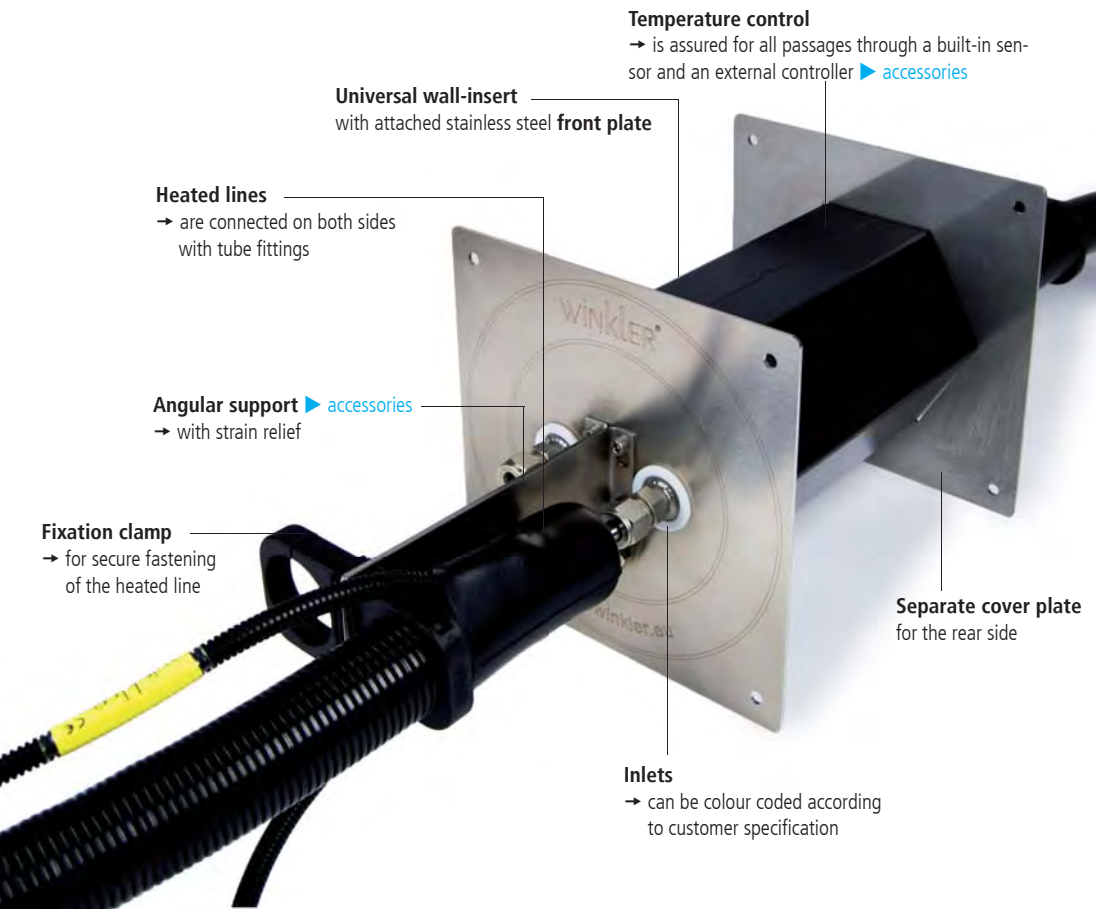
1. Installation of the wall-insert in the wall
