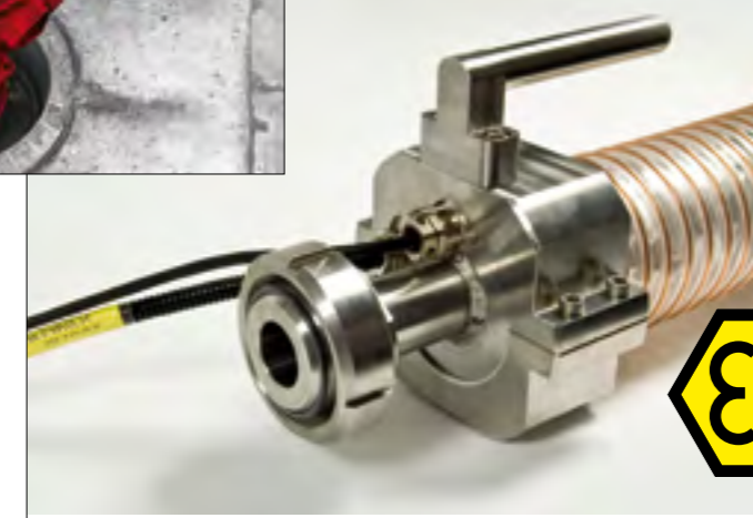
Heated Hoses for filling and dosing systems, transport and discharging technology ATEX Heated Hoses for zones 1/2 (gas) and 21/22 (dust) with EC-type examination certificate
