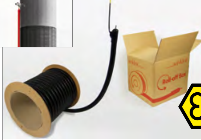
Heated Lines for the process analysis and environmental measurement (emission, imission). Atex Heated Lines for zones 1/2 (gas) and 21/22 (dust) with EC-type examination certificate
