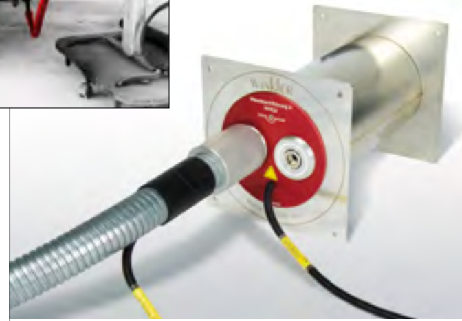
Heated Lines and Heated Wall Bushings for the engine emissions measurement on test beds and vehicles
